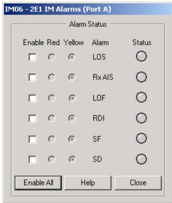
Figure 8 – E1 IM Alarm Monitor Setup Window
