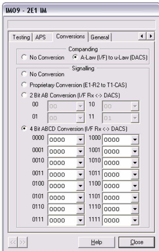
Figure 6 – Dual E1 IM Configuration Dialog Conversion Tab
